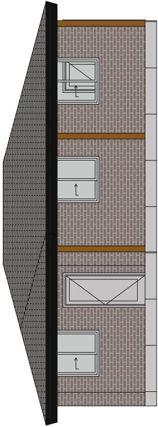
East Elevation 1:100
