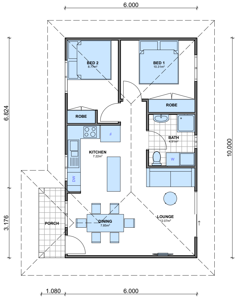
Ground Floor 1:100
