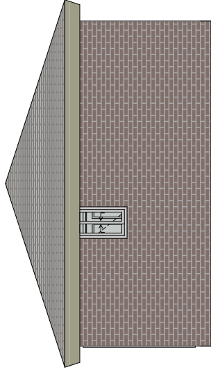
West Elevation 1:100
