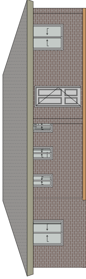
South Elevation 1:100
