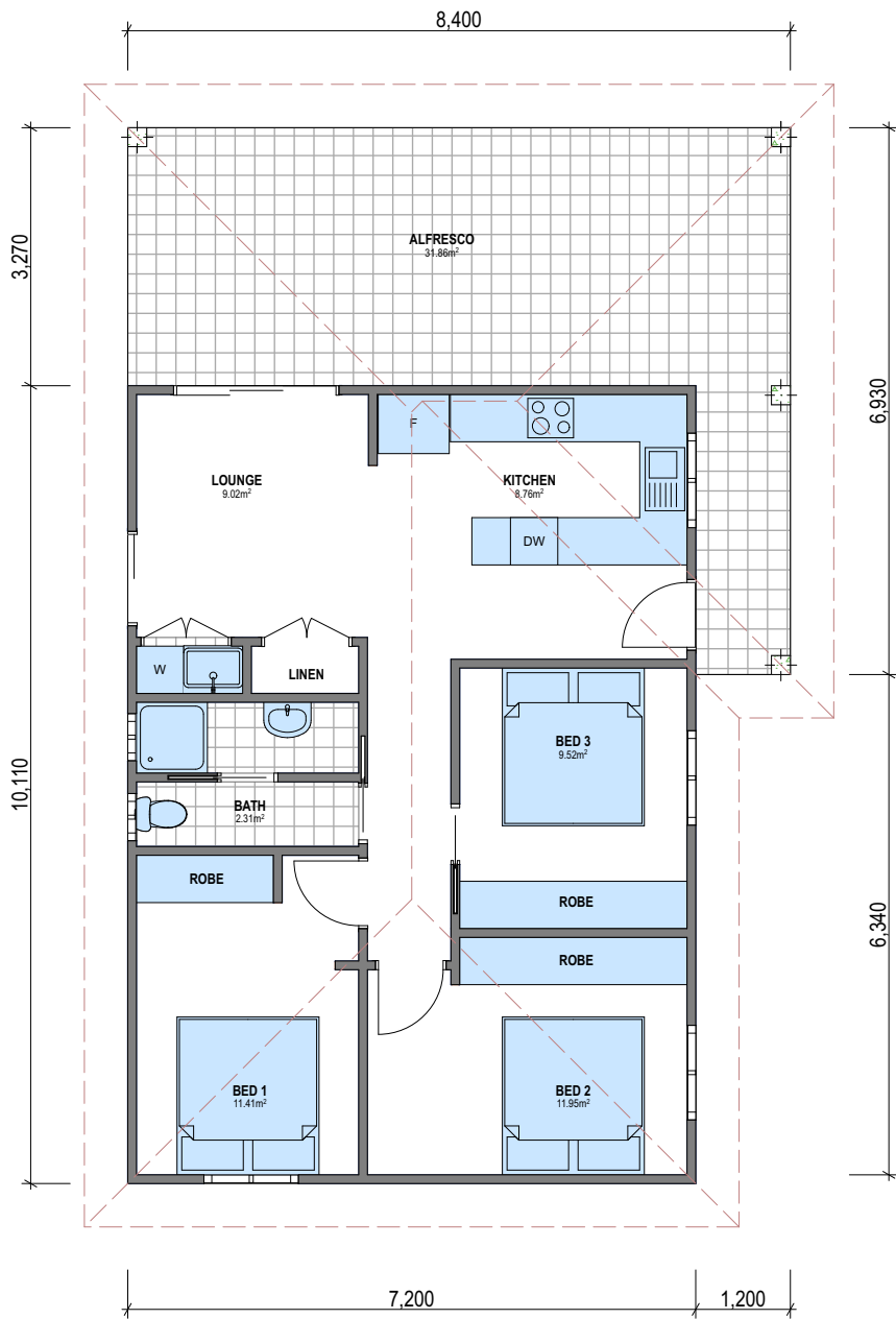
1. GROUND FLOOR PLAN 1:100
