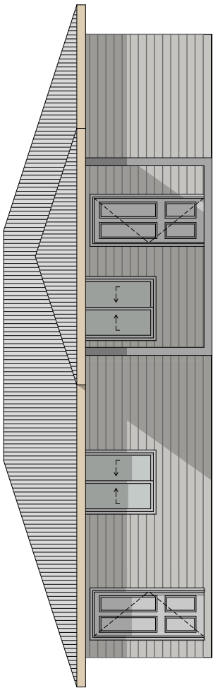
NORTH ELEVATION 1:100
