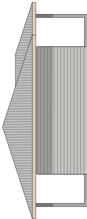
EAST ELEVATION 1:100
