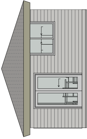
East Elevation 1:100
