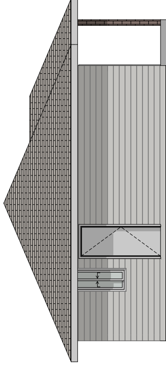
WEST ELEVATION 1:100
