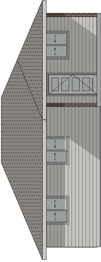
SOUTH ELEVATION 1:100
