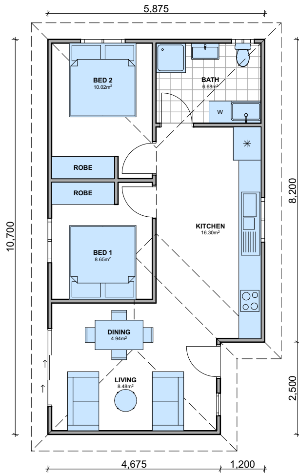
Ground Floor 1:100
