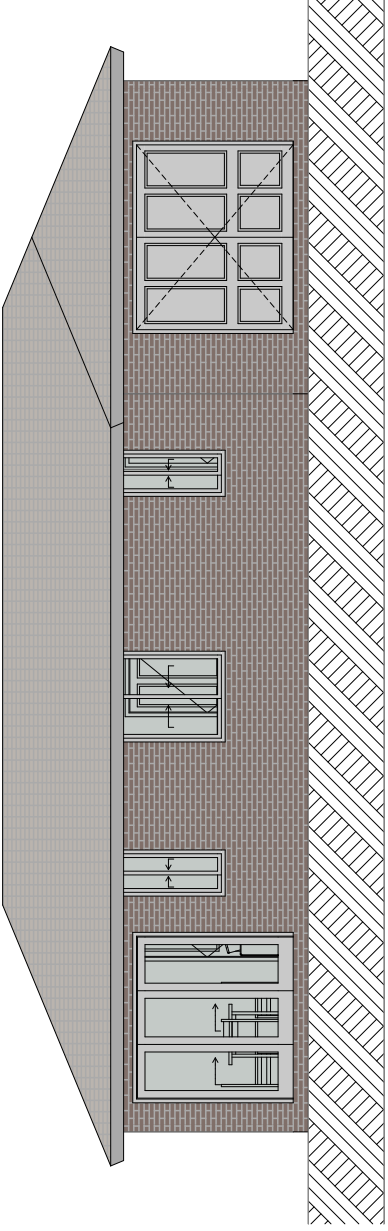
East Elevation 1:100
