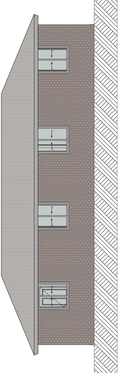
West Elevation 1:100
