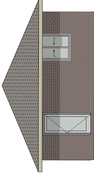
EAST ELEVATION 1:100
