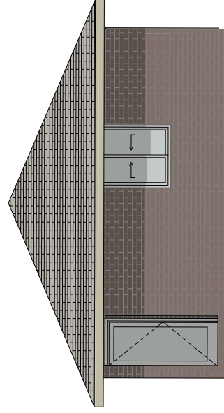
WEST ELEVATION 1:100
