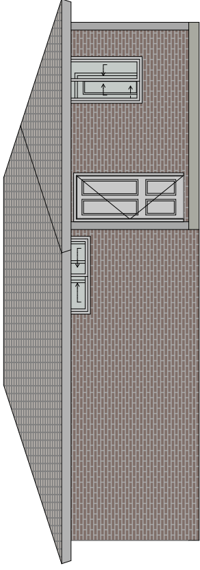
1:100 East Elevation
