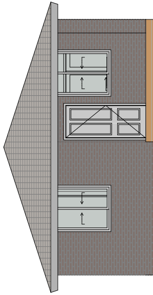
South Elevation 1:100
