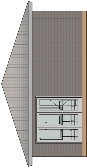
North Elevation 1:100
