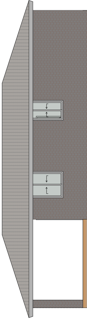
West Elevation 1:100
