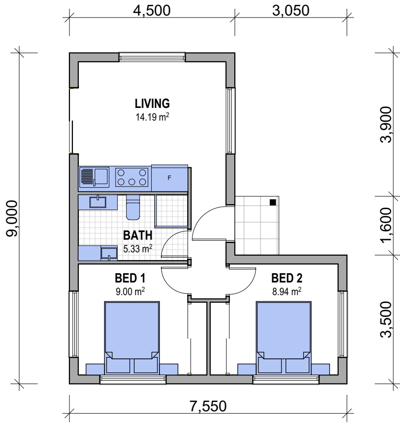
GRN FLAT - FLOOR PLAN
