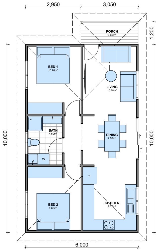
Ground Floor 1:100
