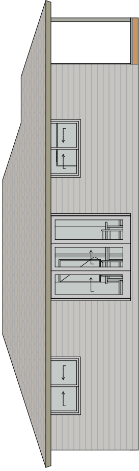
East Elevation 1:100
