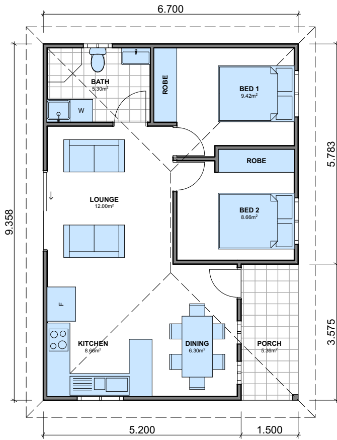
1:100 Ground Floor
