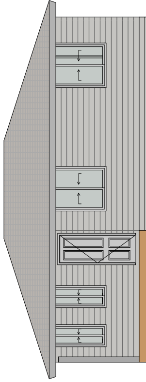
1:100 East Elevation
