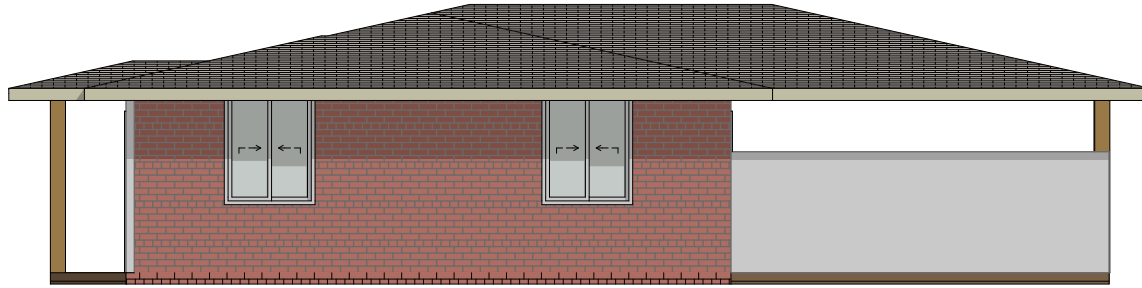
NORTH ELEVATION (1) 1:100
