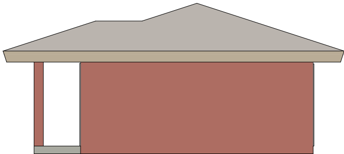
South Elevation 1:100
