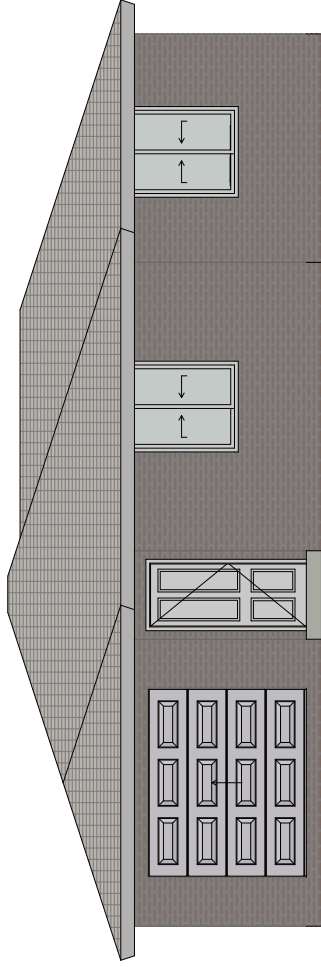
South Elevation 1:100
