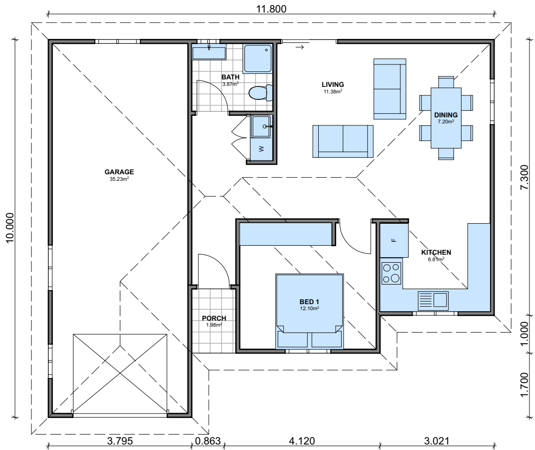
Ground Floor
