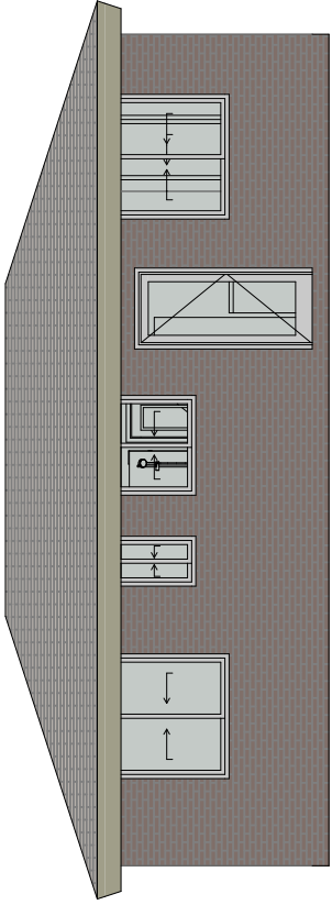
North Elevation 1:100
