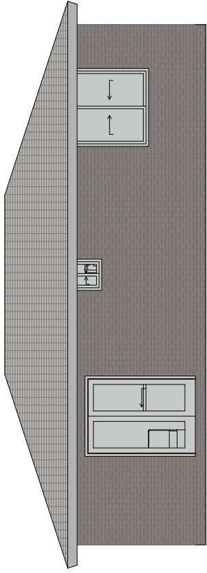
North Elevation 1:100
