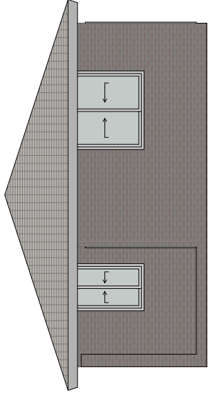
East Elevation 1:100
