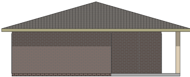
NORTH ELEVATION 1:100
