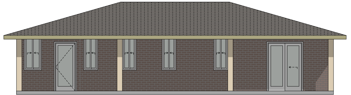
WEST ELEVATION 1:100
